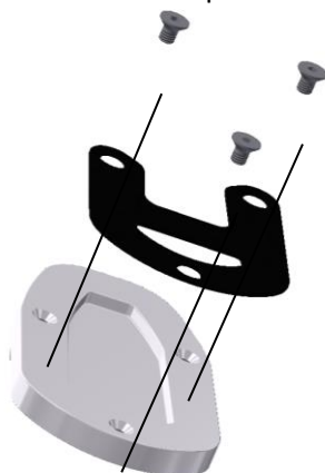
ASSEMBLY VIEW
