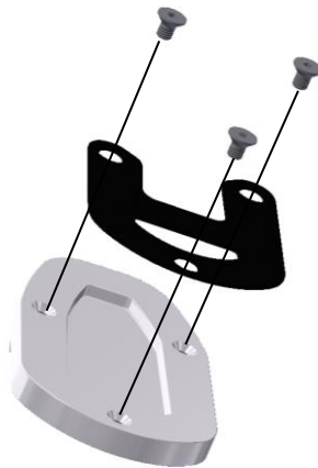
ASSEMBLY VIEW
